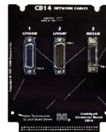
CB14 Molex LFH Connectors (Item 744)
