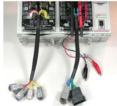
Adapter Cables, with Alligator Clips to Accept Lugs on Flying Leads
