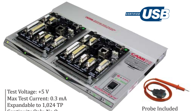
CableEye M2U (Item 811U) with CB15 Boards (Item 745) Installed
