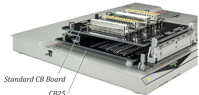
CB25B Right-Angle Transition Board (Item 755B)
