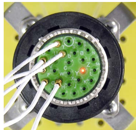
AutoBuild with the Light Director Setup for 1st-Sided pinning. Target cavity is illuminated from below with LED light fiber. See "Light-Guided Assembly" on p.30.
