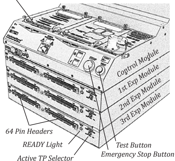
HVX System with Three Expansion Modules
