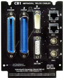
CB1 CN50, DB15 RJ45, BNC (Item 731)
