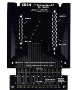
CB44 Micro D Connectors, 51- and 100-Pin (Item 774)
