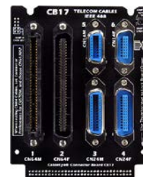
CB17 Telecom Connectors, IEEE 488 (Item 747)
