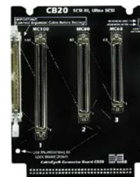
CB20 (Item 750) (mini-Centronics)
